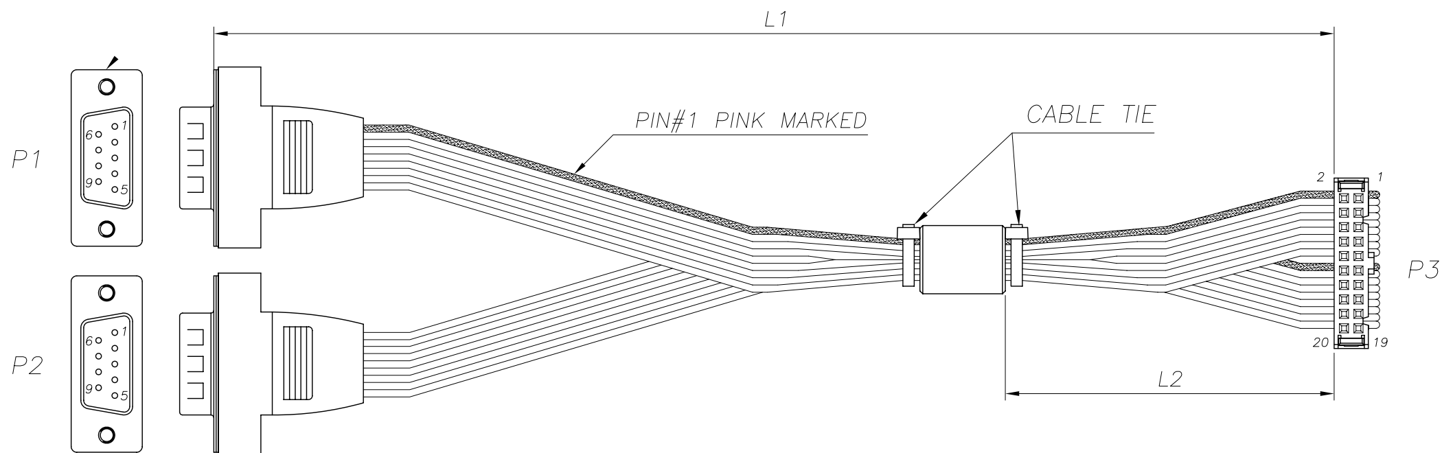
WIRE DIAGRAM
