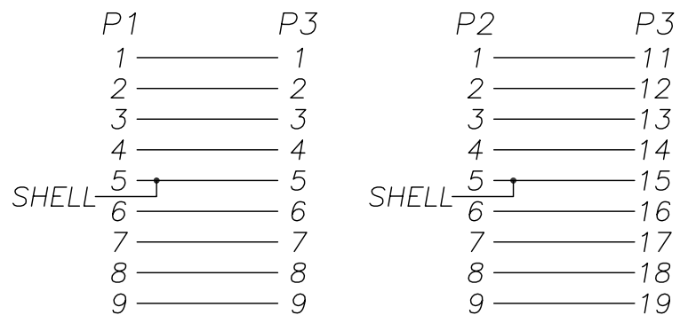
WIRE DIAGRAM
