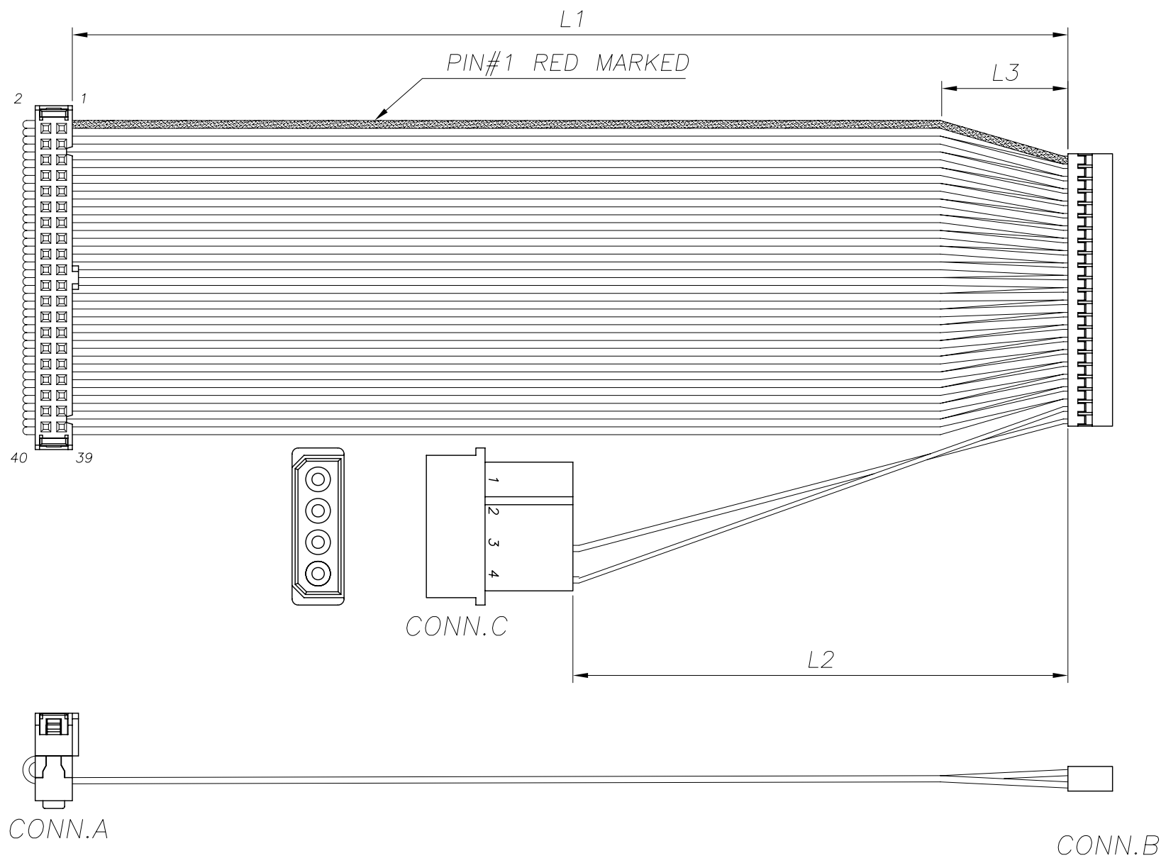
WIRE DIAGRAM
